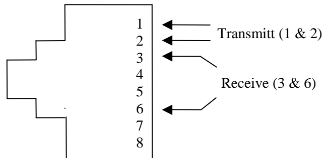
Figure 2. BES 10 NTE - RJ45 Connector Pin Out Connections
